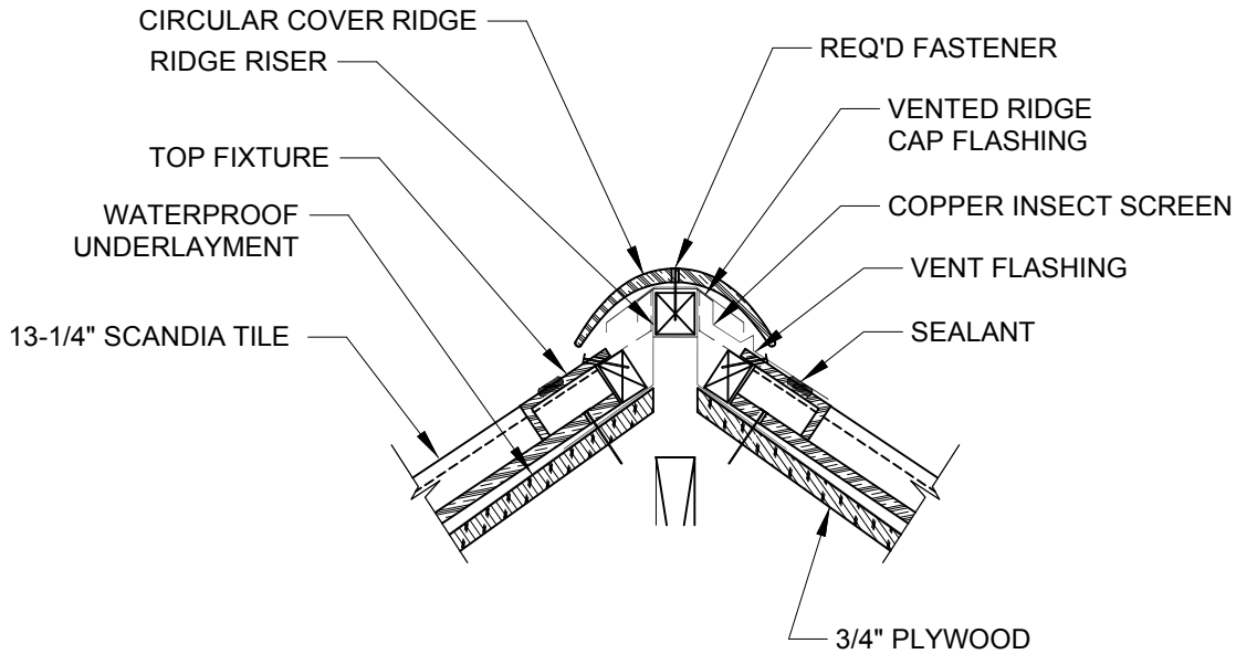
SECTION AT CIRCULAR COVER VENTED RIDGE WITH TOP FIXTURE SCALE 1-1/2" = 1'
